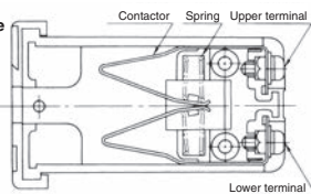
Diagram of contactor for voltage (KTT-VS□)
