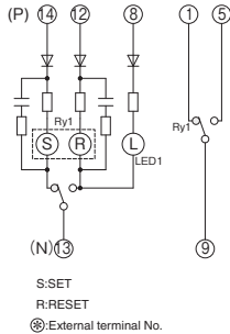
[1c contact specification]
